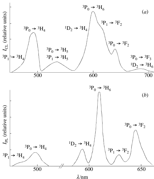
Figure 1 PL and CL spectra: (a) CL spectra of 10^{-2} \text{ M} AAD in the presence of 7 \times 10^{-2} \text{ M} \text{Pr}(\text{fod})_3 at 90^\circ\text{C} in toluene (spectral slit \Delta\lambda = 7 \text{ nm} ); (b) PL spectra of 10^{-2} \text{ M} \text{Pr}(\text{L})_3 in [\text{2H}_8]\text{toluene} at room temperature, \lambda_{\text{ex}} = 370 \text{ nm} (spectral slit \Delta\lambda = 5 \text{ nm} ).
