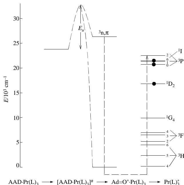
Figure 2 Energy scheme for AAD decomposition in the complex \text{Pr}(\text{L})_3\cdot\text{AAD} . The energy of the triplet adamantanone 11 E_T = 75.2 \text{ kcal mol}^{-1} ; the enthalpy of decomposition of 1,2-dioxetane 12 is \Delta H \approx 68 \text{ kcal mol}^{-1} . Photo- and chemiluminescence are observed from the \text{Pr}^{3+} levels marked by (•).
